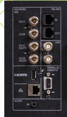
REAR PANEL
